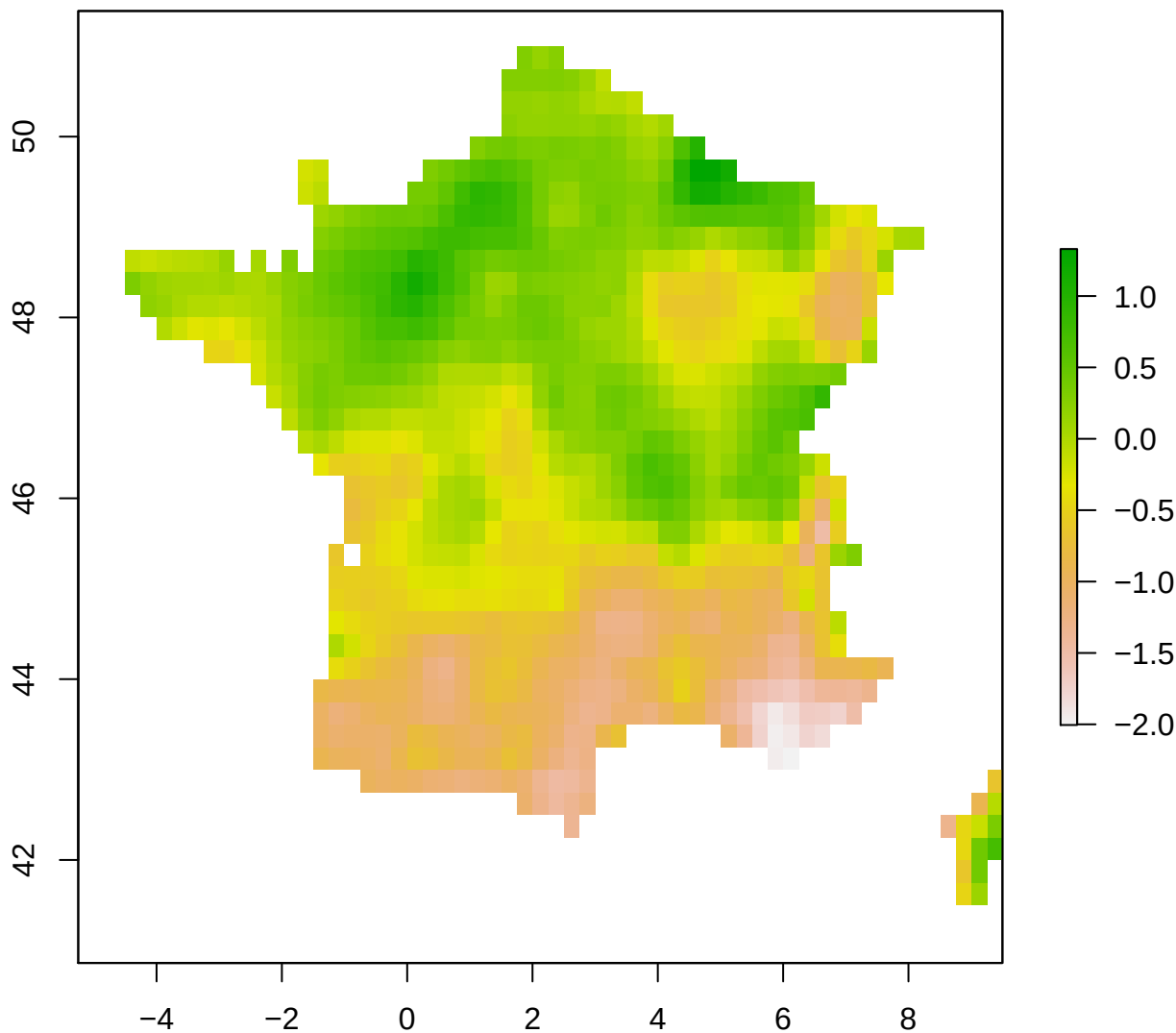
spi12_month – France 2008-02-01
