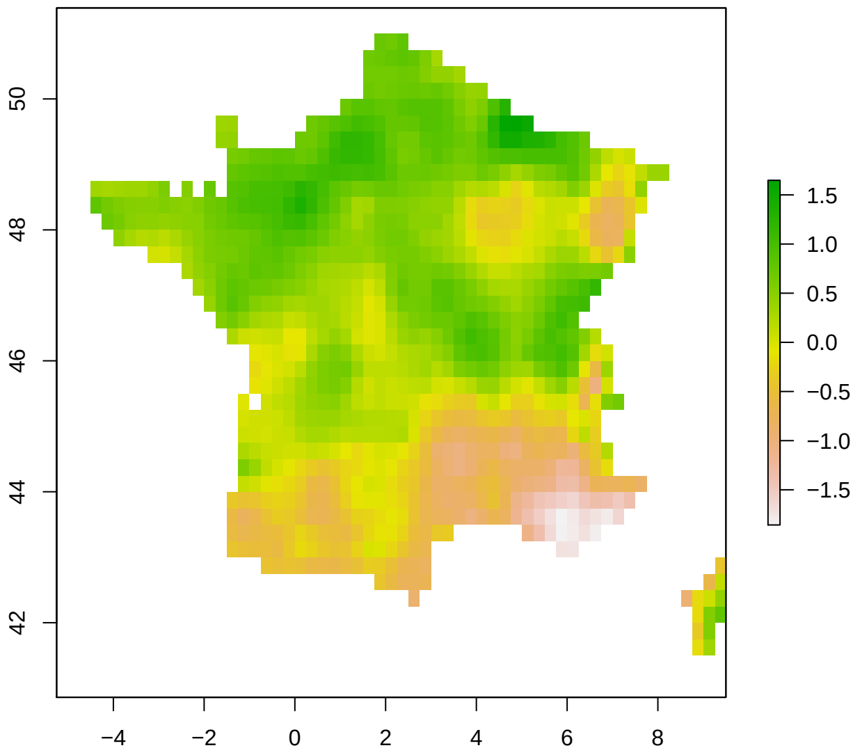
spi12_month – France 2008-01-01
