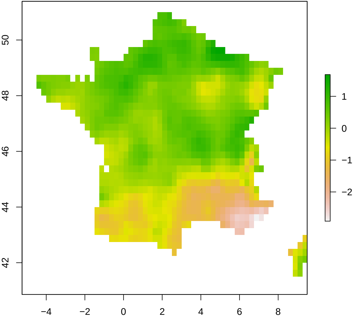
spi12 month – France 2007-12-01
