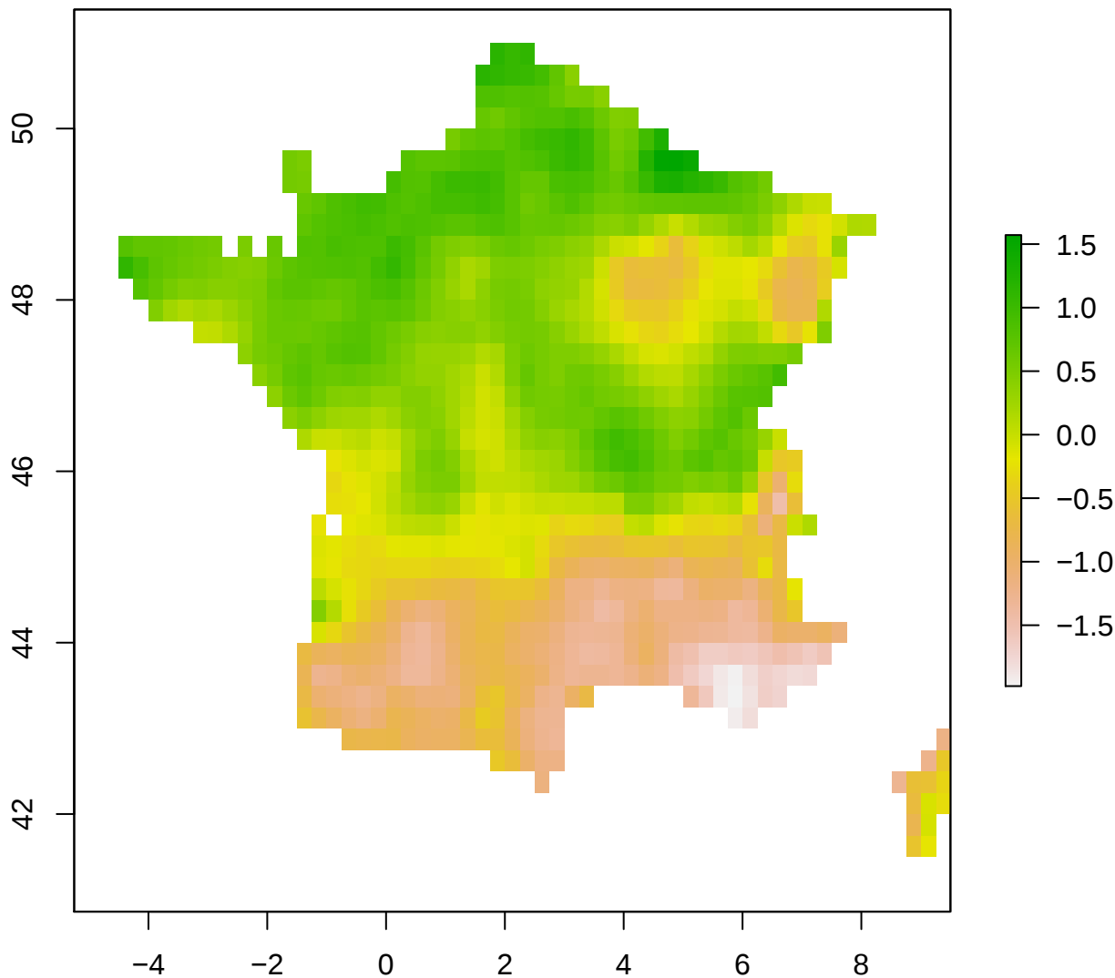
spi12_month – France 2007-11-01
