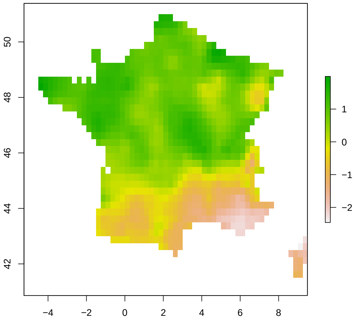
spi12_month – France 2007-09-01
