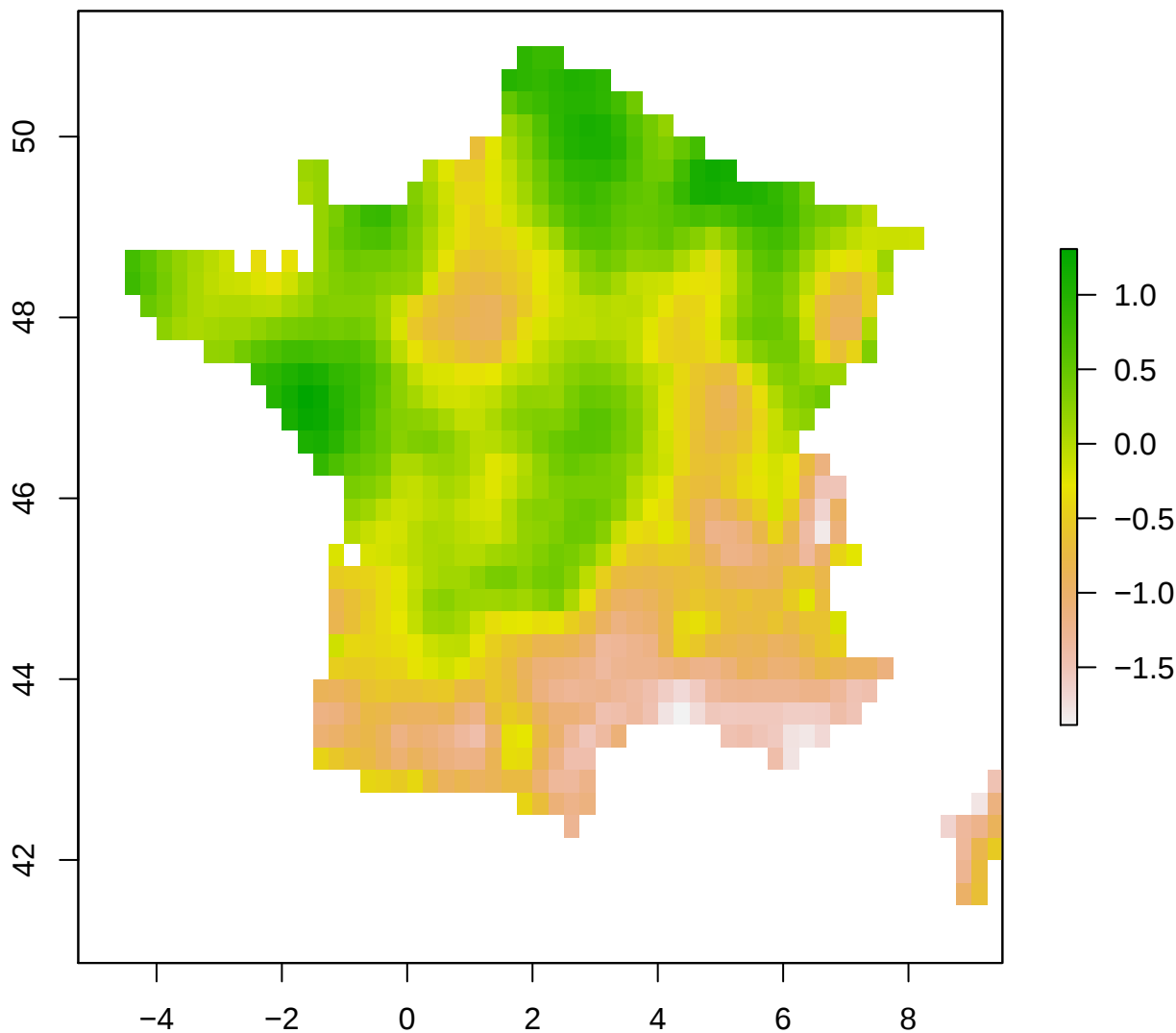
spi12_month – France 2007-04-01
