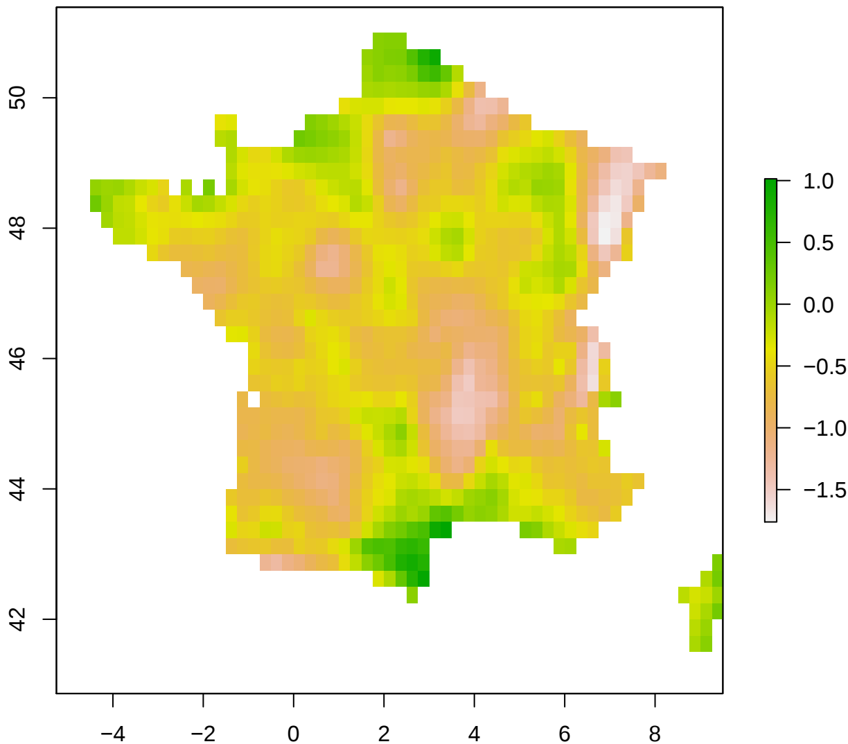
spi12_month – France 2006-03-01
