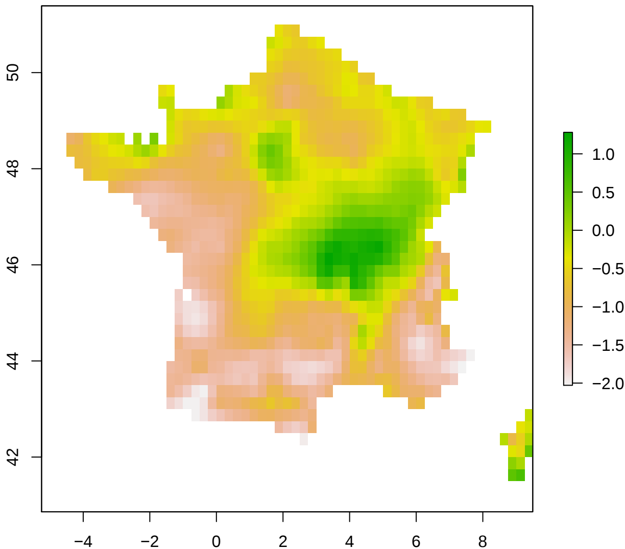
spi12_month – France 2005-06-01
