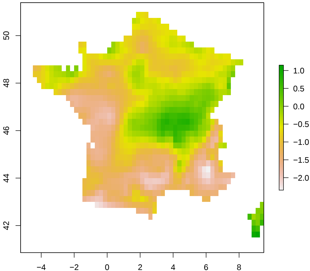
spi12_month – France 2005-04-01
