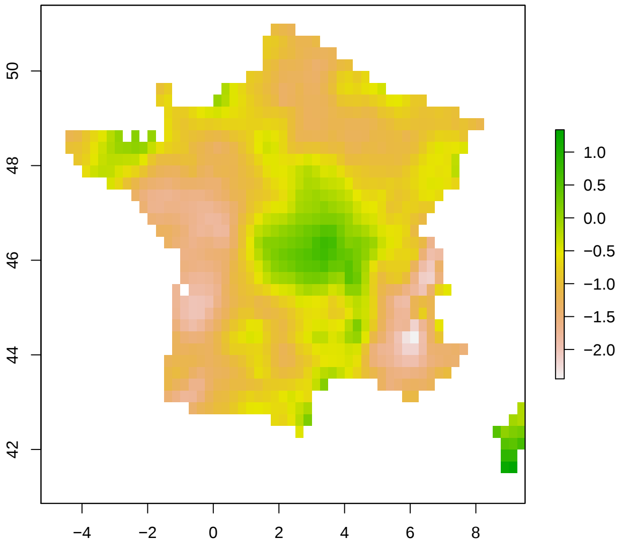
spi12_month – France 2005-01-01
