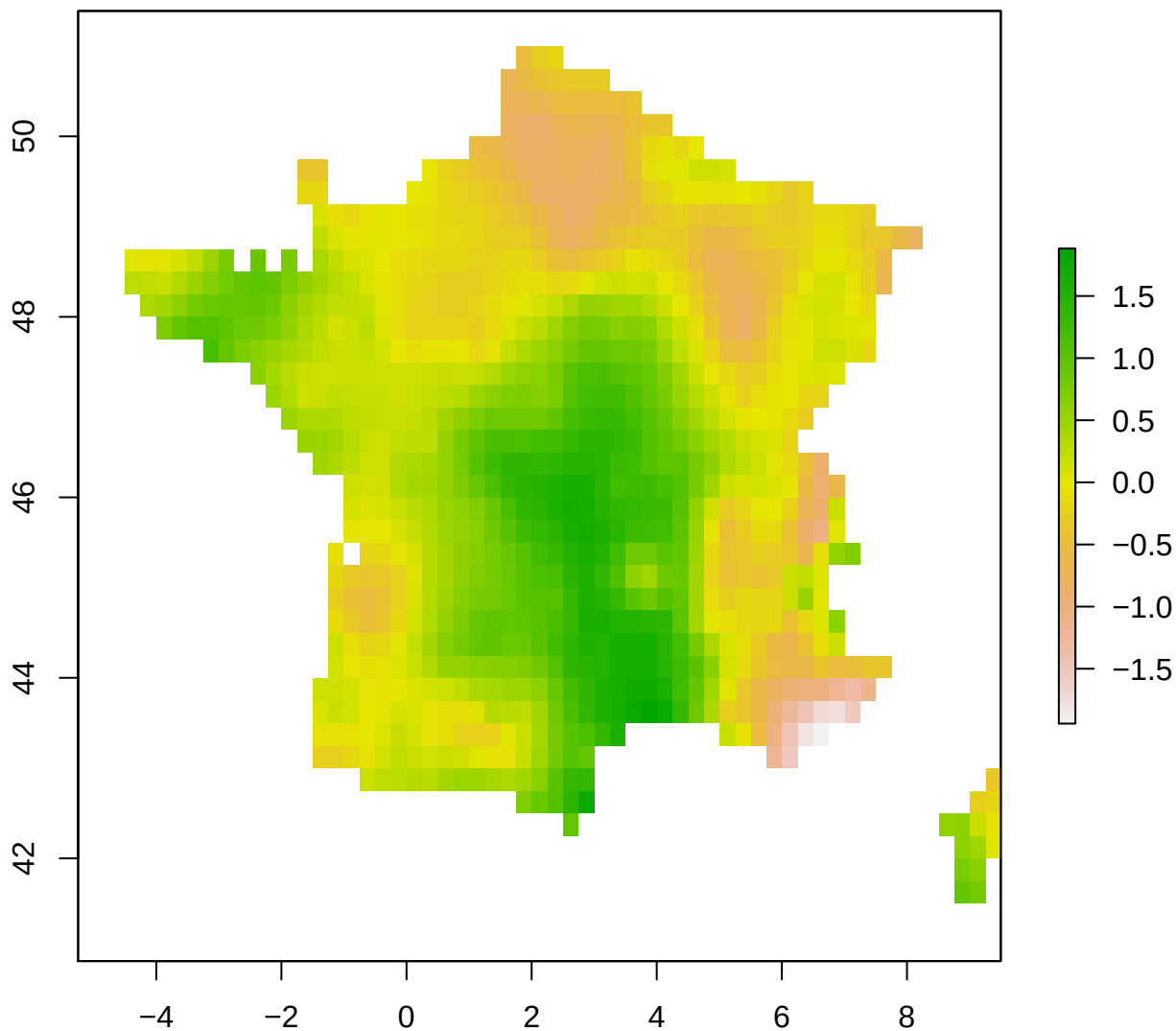
spi12_month – France 2004-08-01
