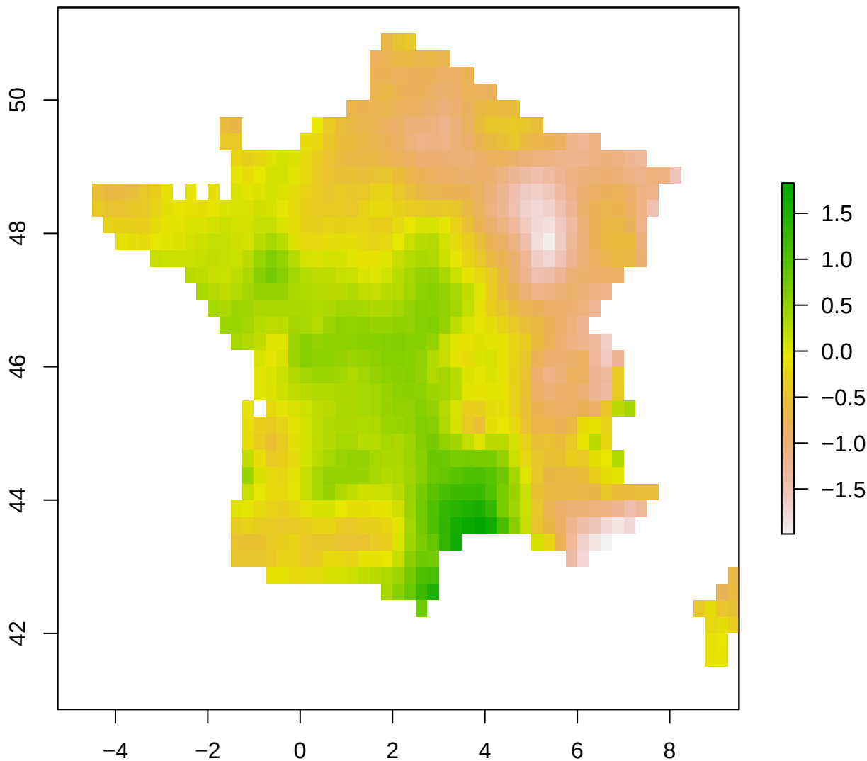
spi12_month – France 2004-04-01
