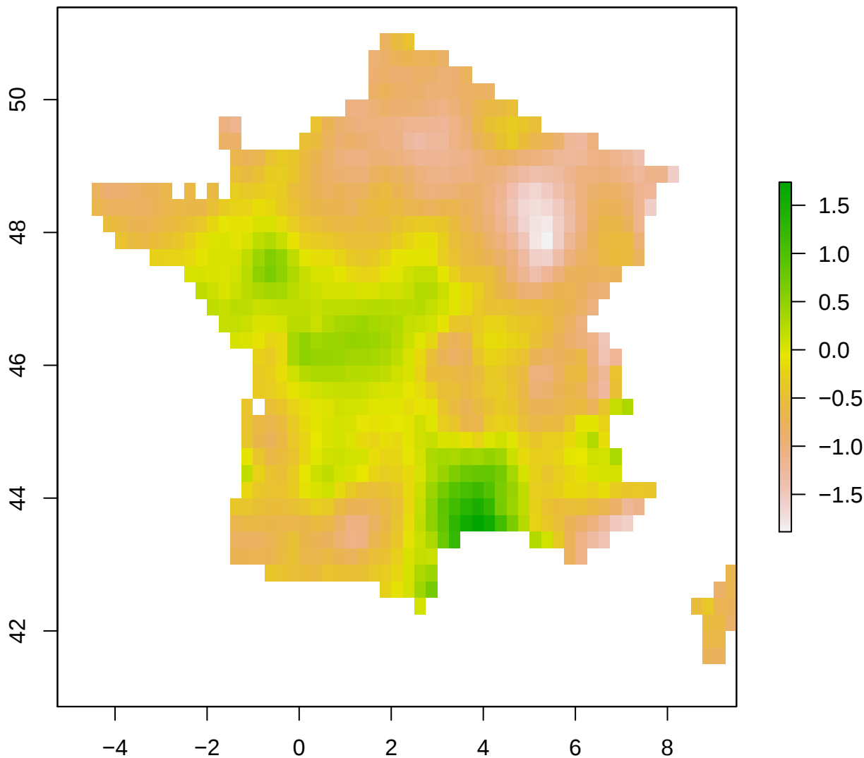
spi12_month – France 2004-03-01
