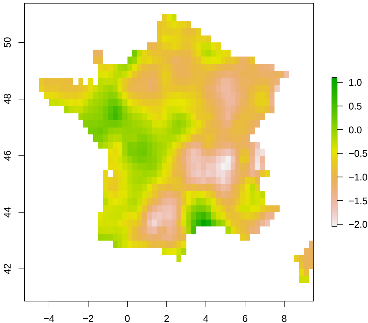
spi12_month – France 2003-11-01
