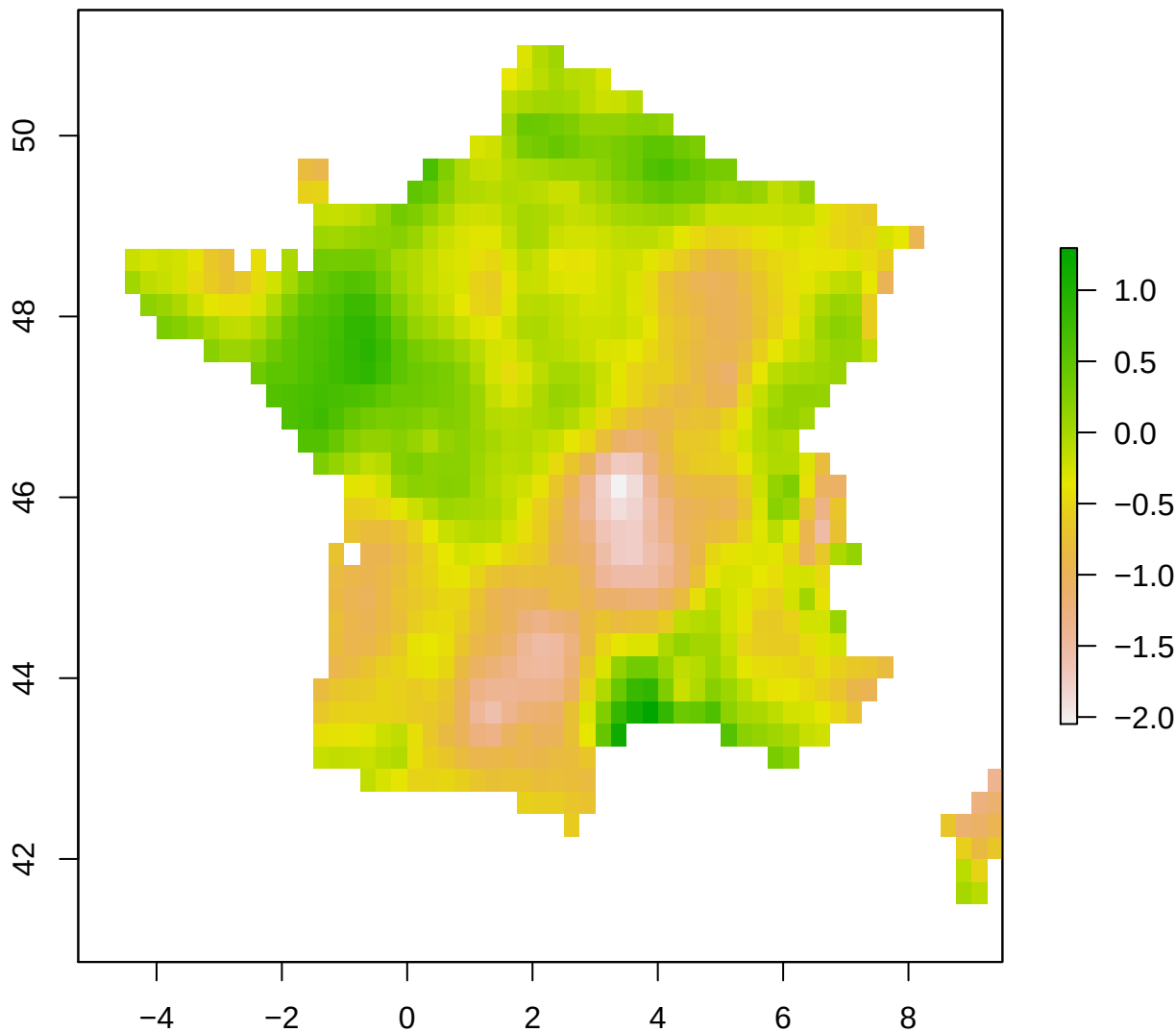
spi12_month – France 2003-09-01
