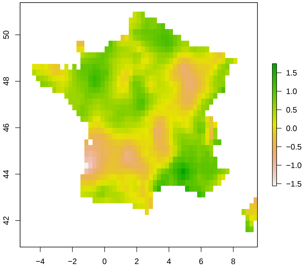
spi12_month – France 2003-05-01
