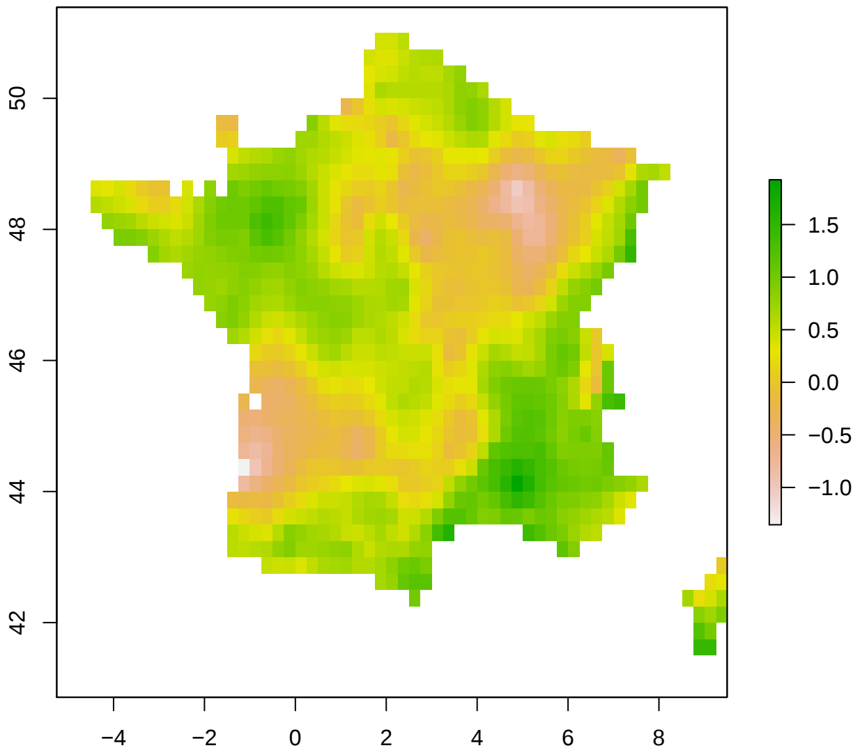
spi12_month – France 2003-03-01
