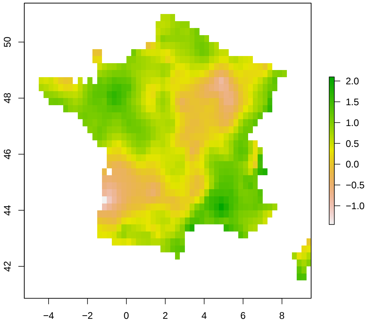
spi12_month – France 2003-02-01
