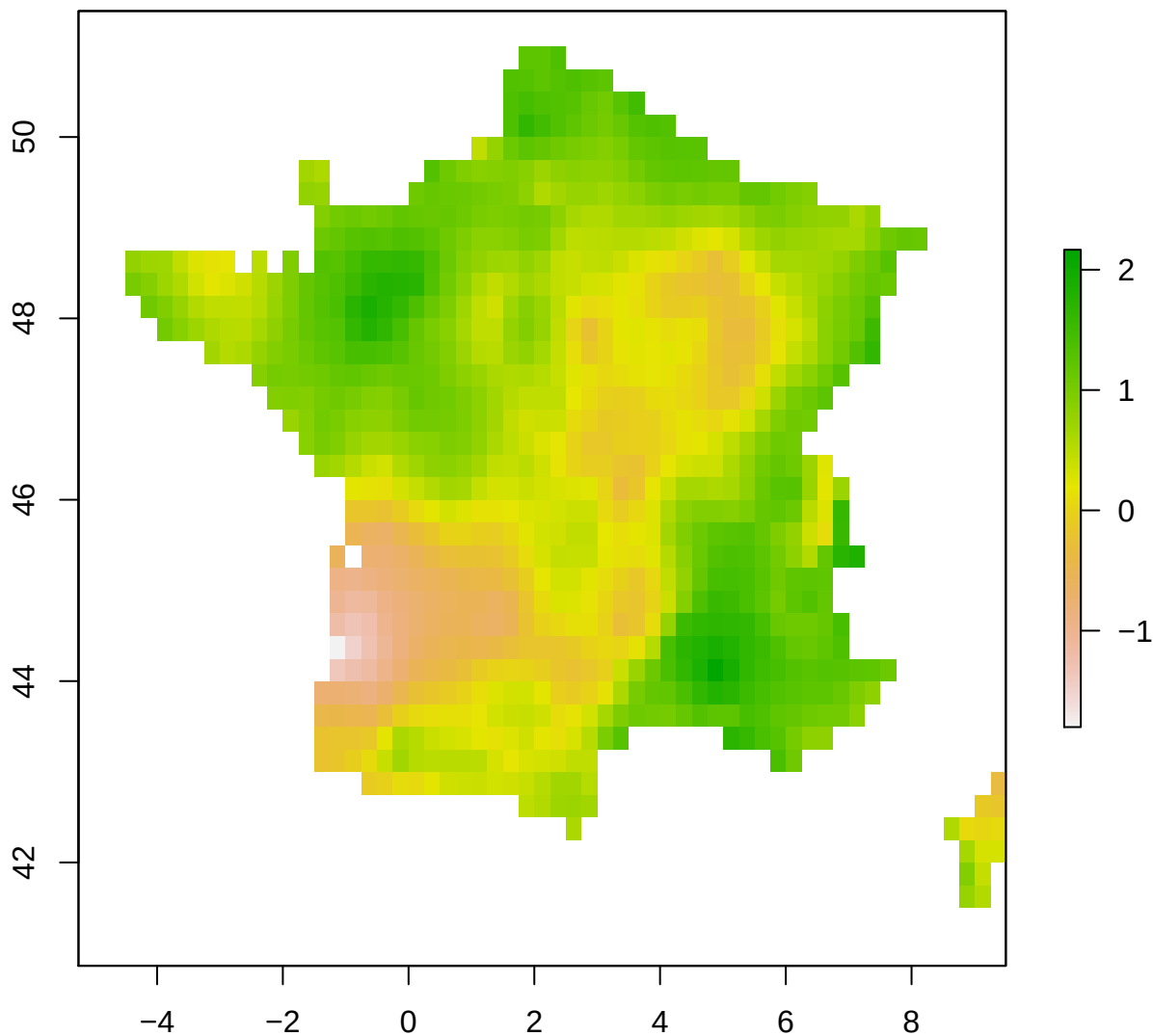
spi12_month – France 2002-12-01
