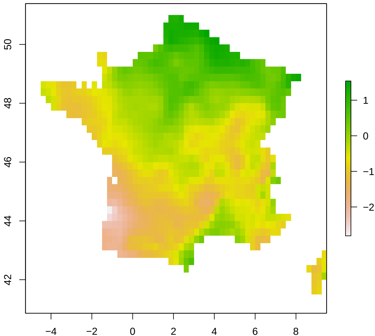
spi12_month – France 2002-08-01
