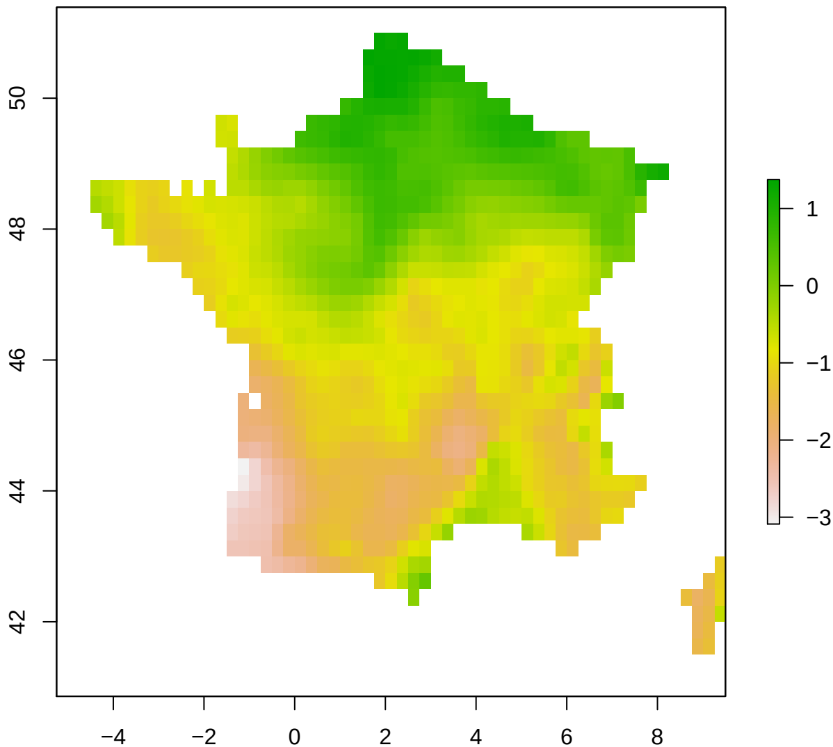
spi12_month – France 2002-07-01
