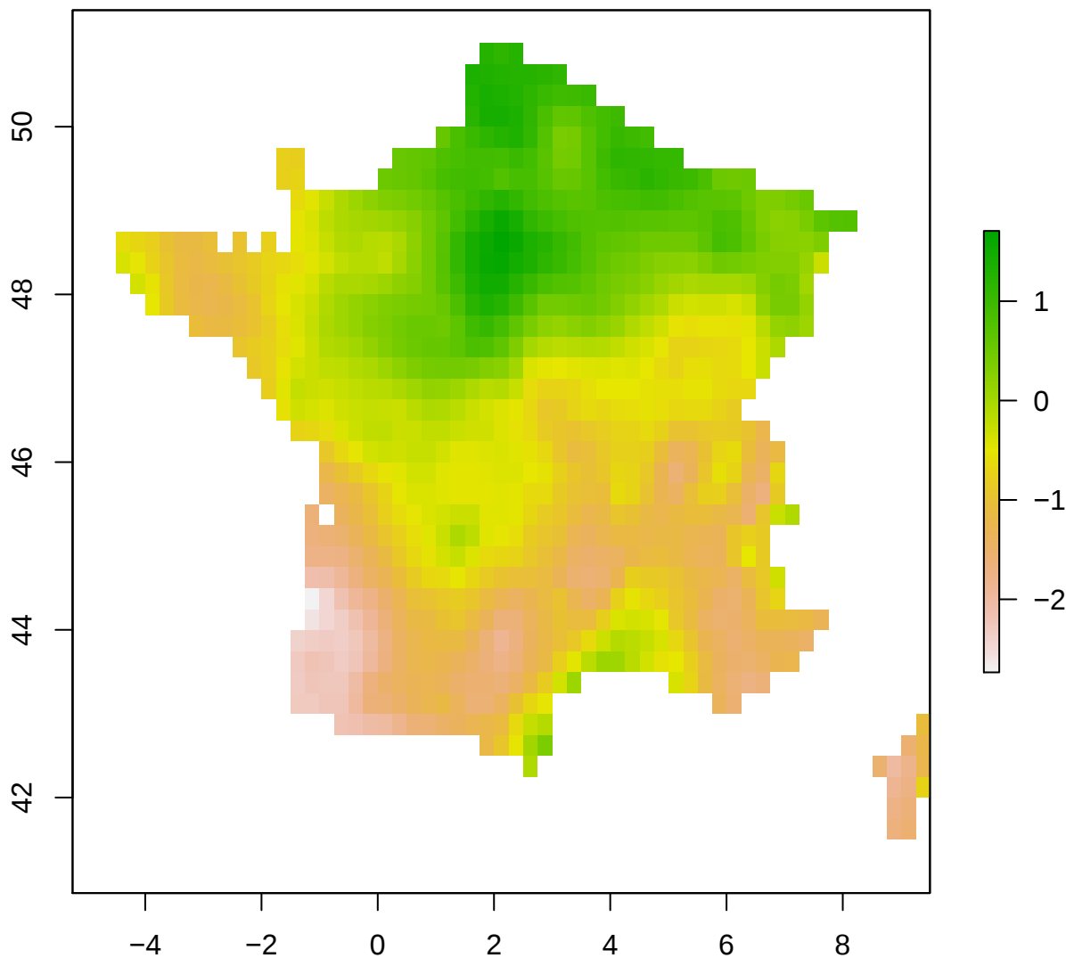
spi12_month – France 2002-06-01
