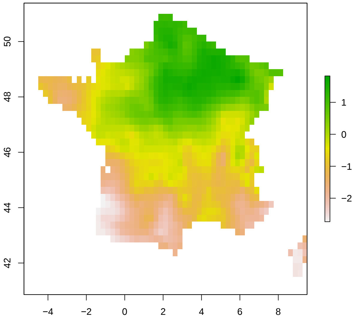
spi12_month – France 2002-03-01
