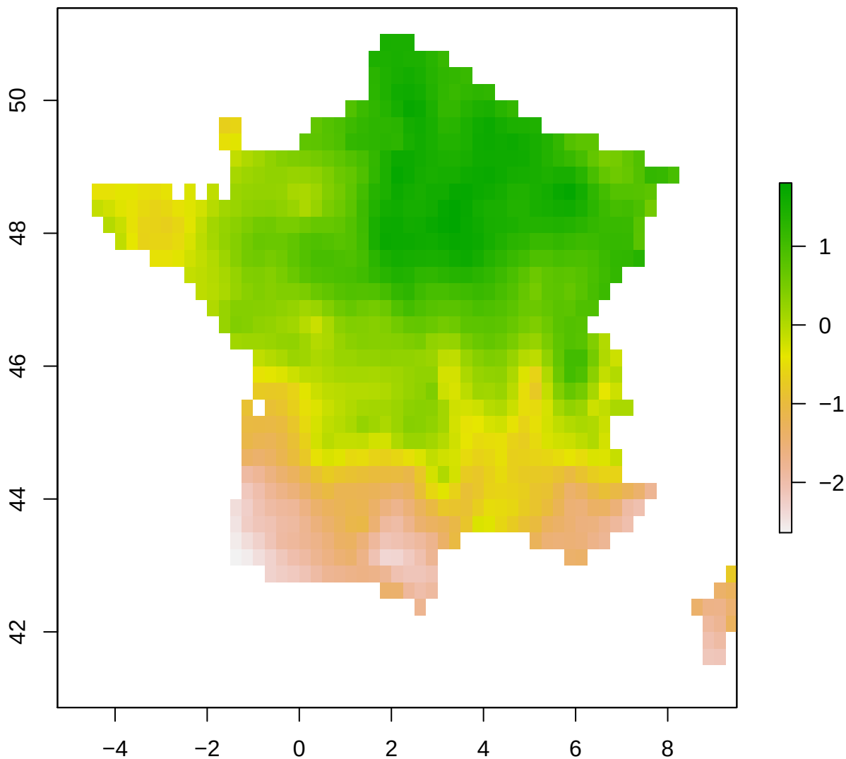
spi12_month - France 2002-01-01
