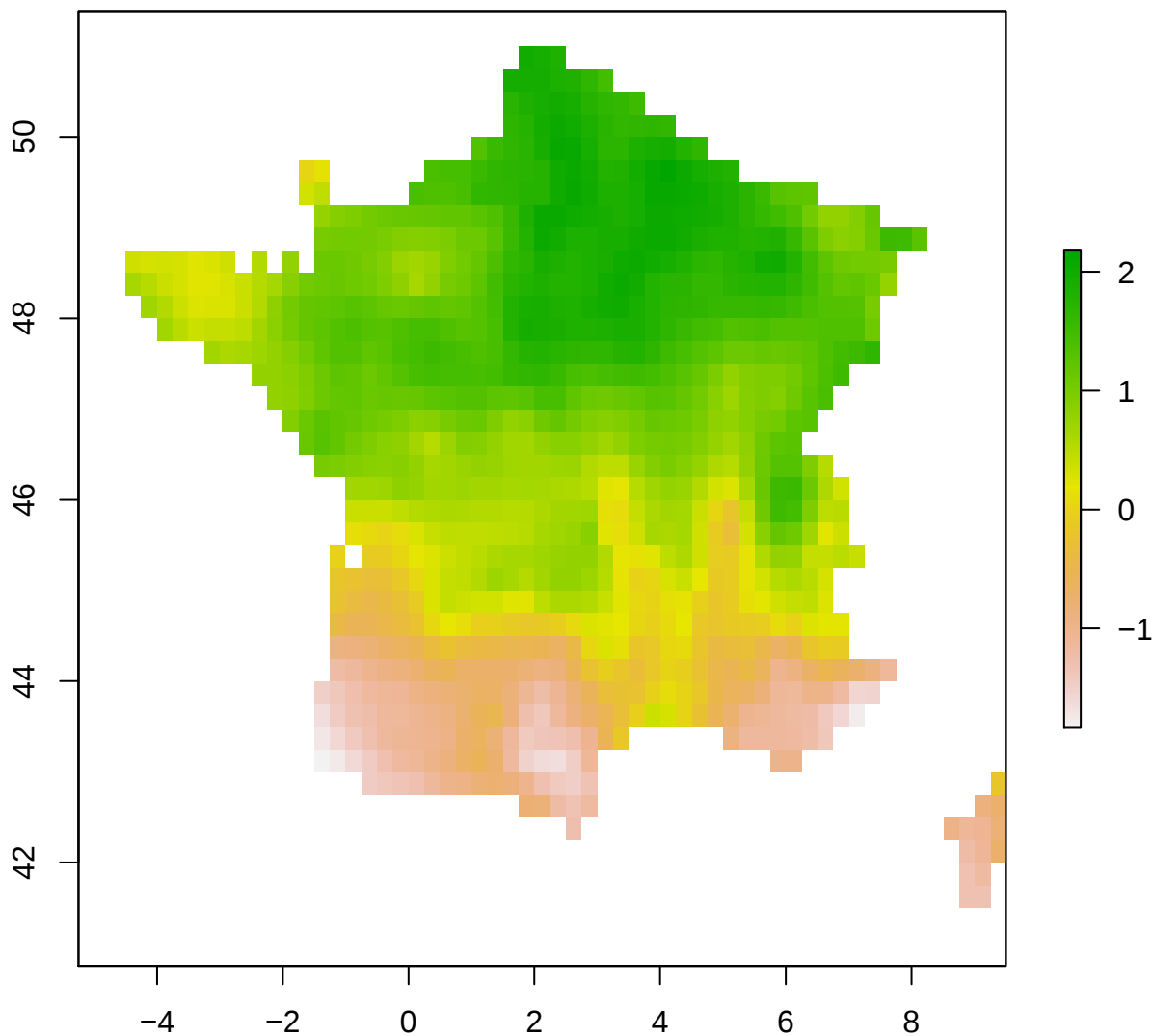
spi12_month – France 2001-12-01
