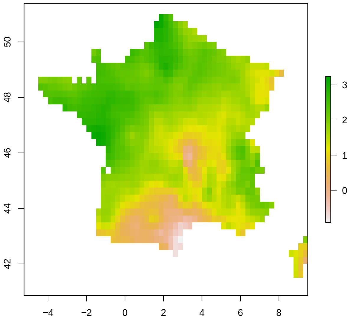
spi12_month – France 2001-08-01
