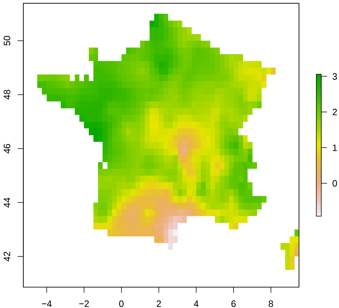
spi12_month – France 2001-07-01
