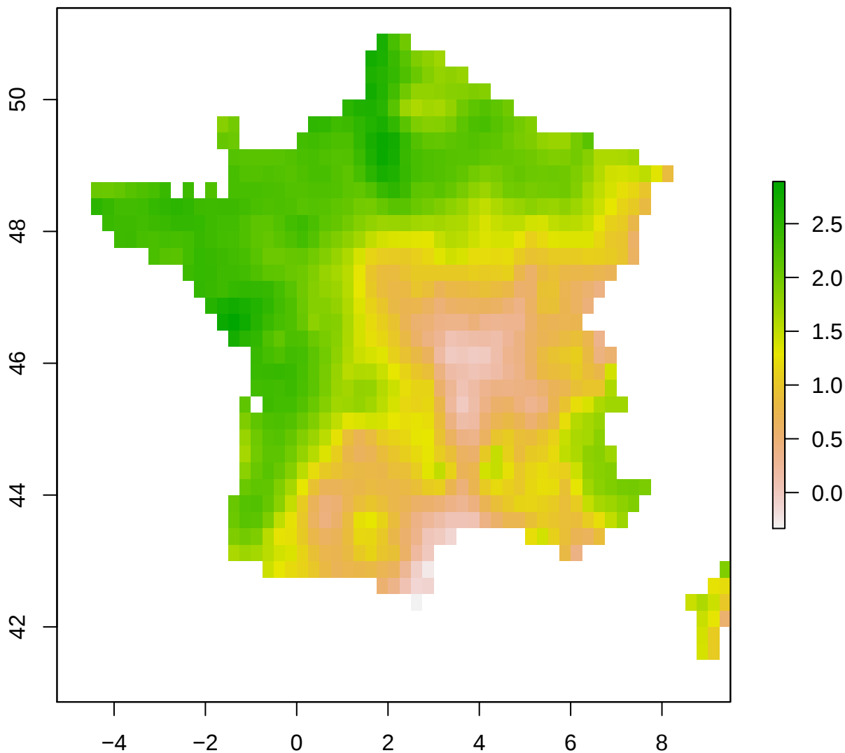
spi12_month – France 2001-01-01
