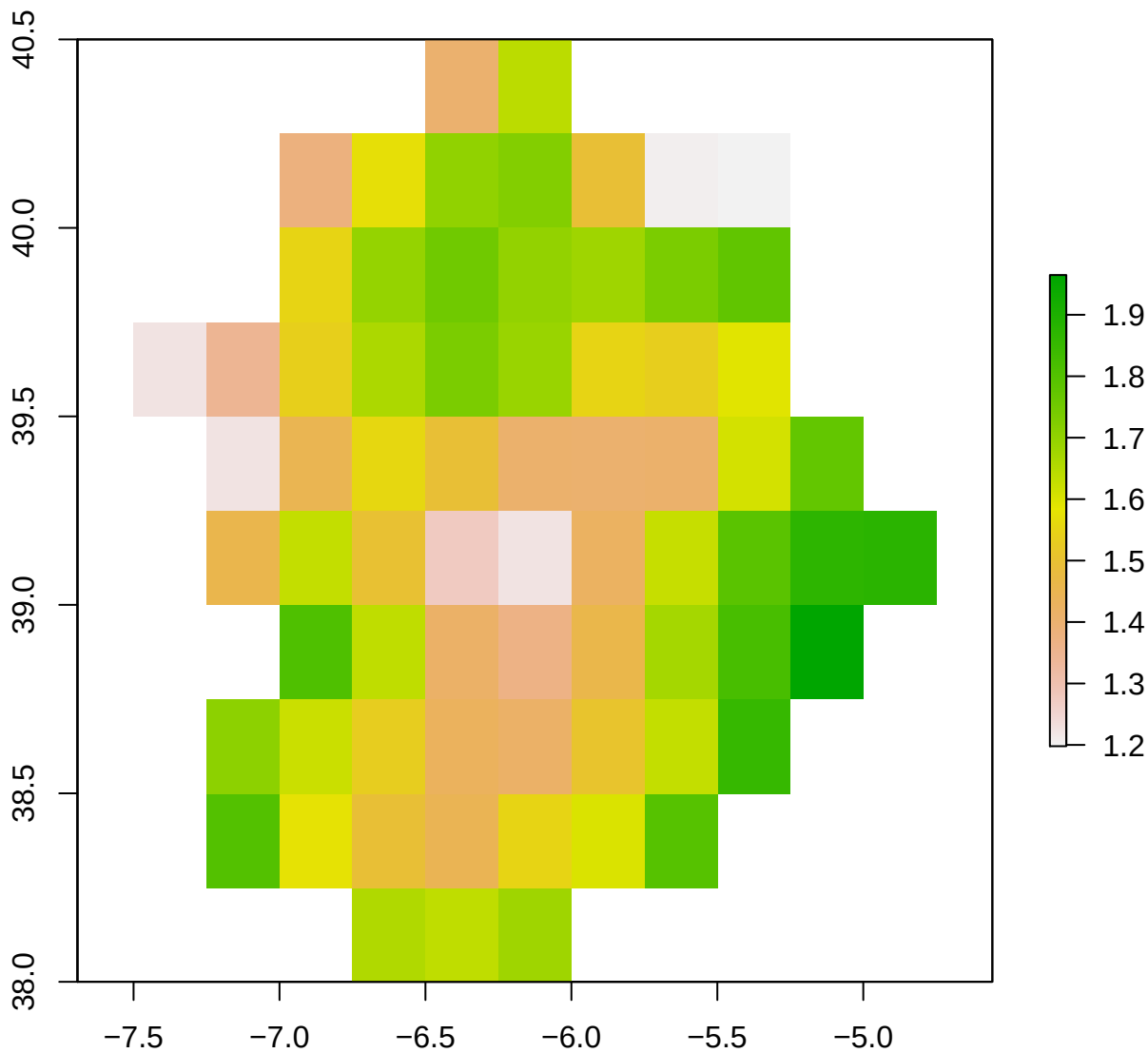
spi12_month - ES43 2010-12-01
