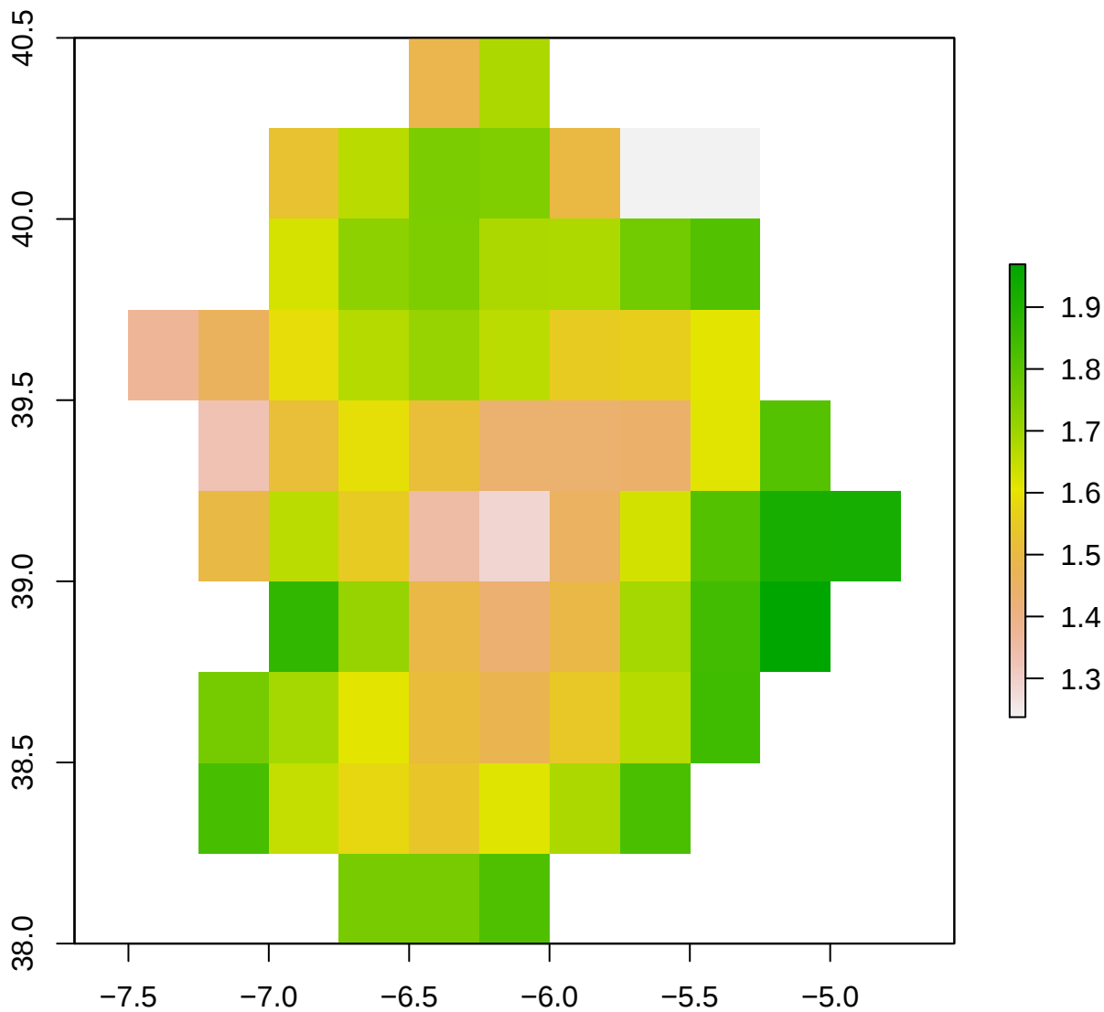
spi12_month - ES43 2010-11-01
