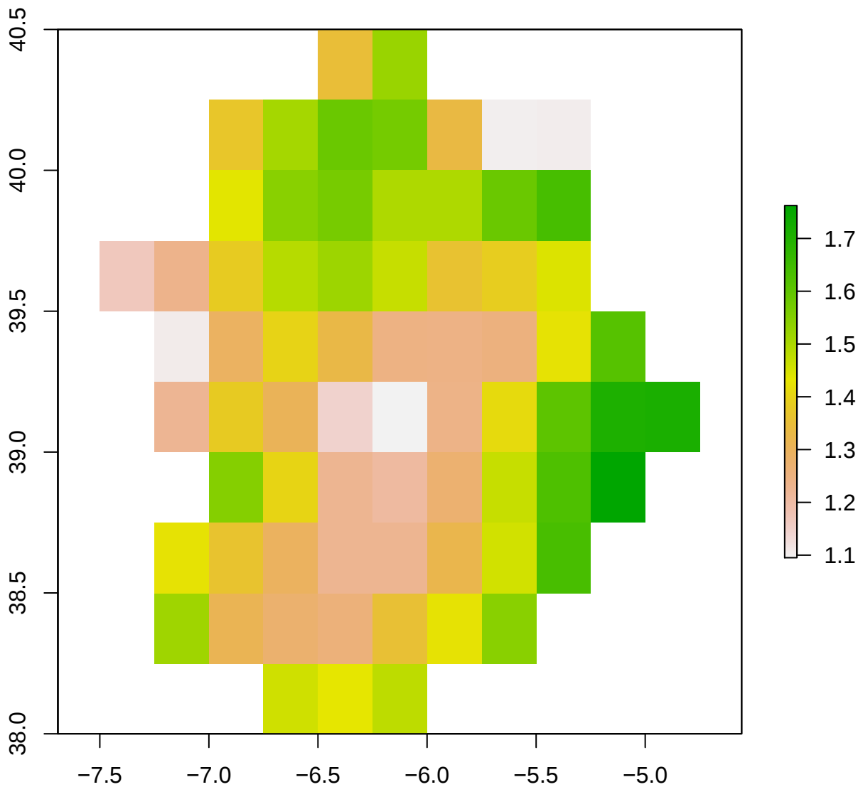
spi12_month - ES43 2010-10-01
