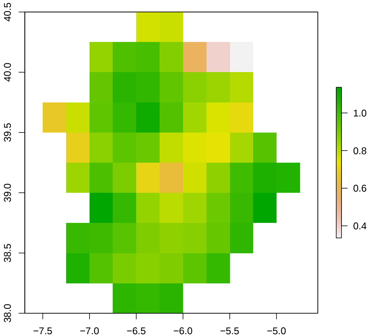
spi12_month - ES43 2010-03-01
