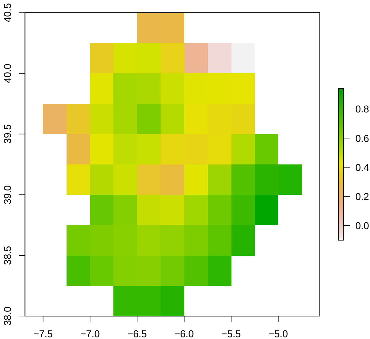
spi12_month - ES43 2010-02-01
