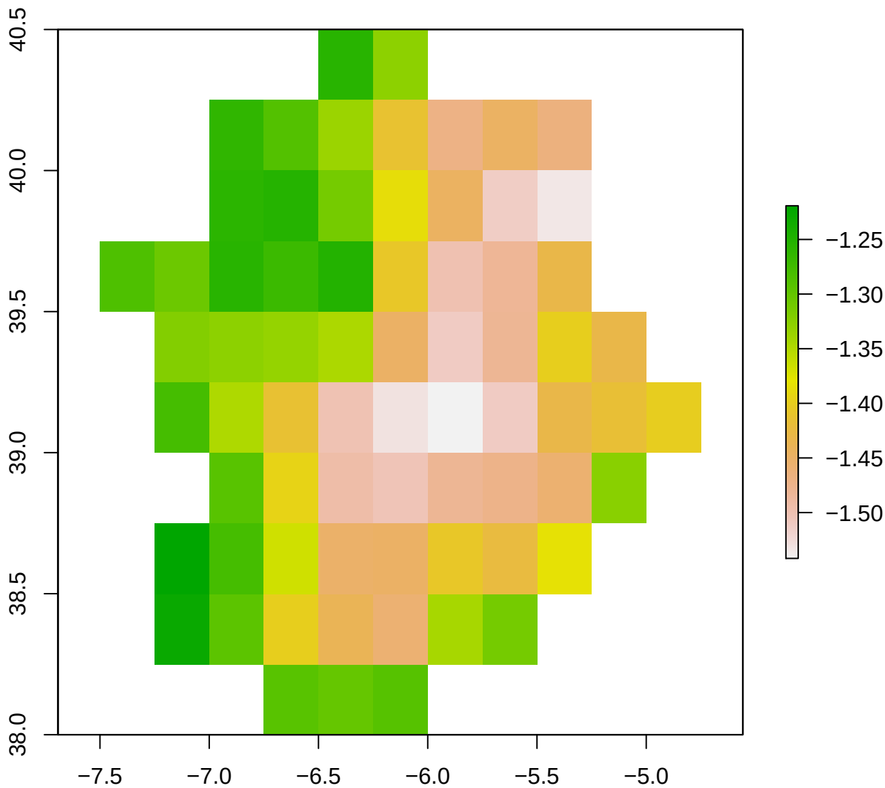
spi12_month - ES43 2009-11-01
