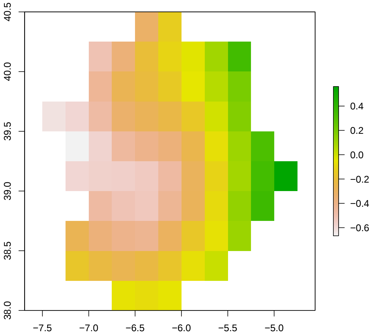
spi12_month - ES43 2009-03-01
