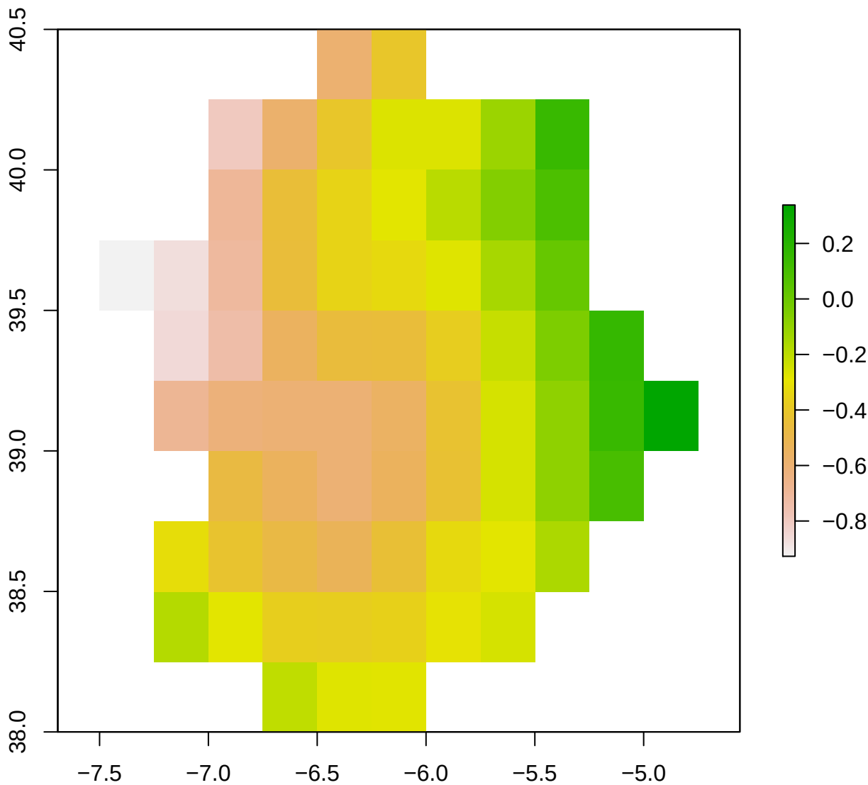
spi12_month - ES43 2008-12-01
