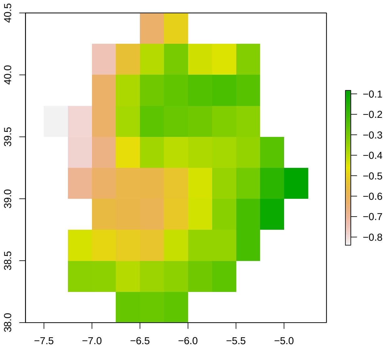
spi12_month - ES43 2008-09-01
