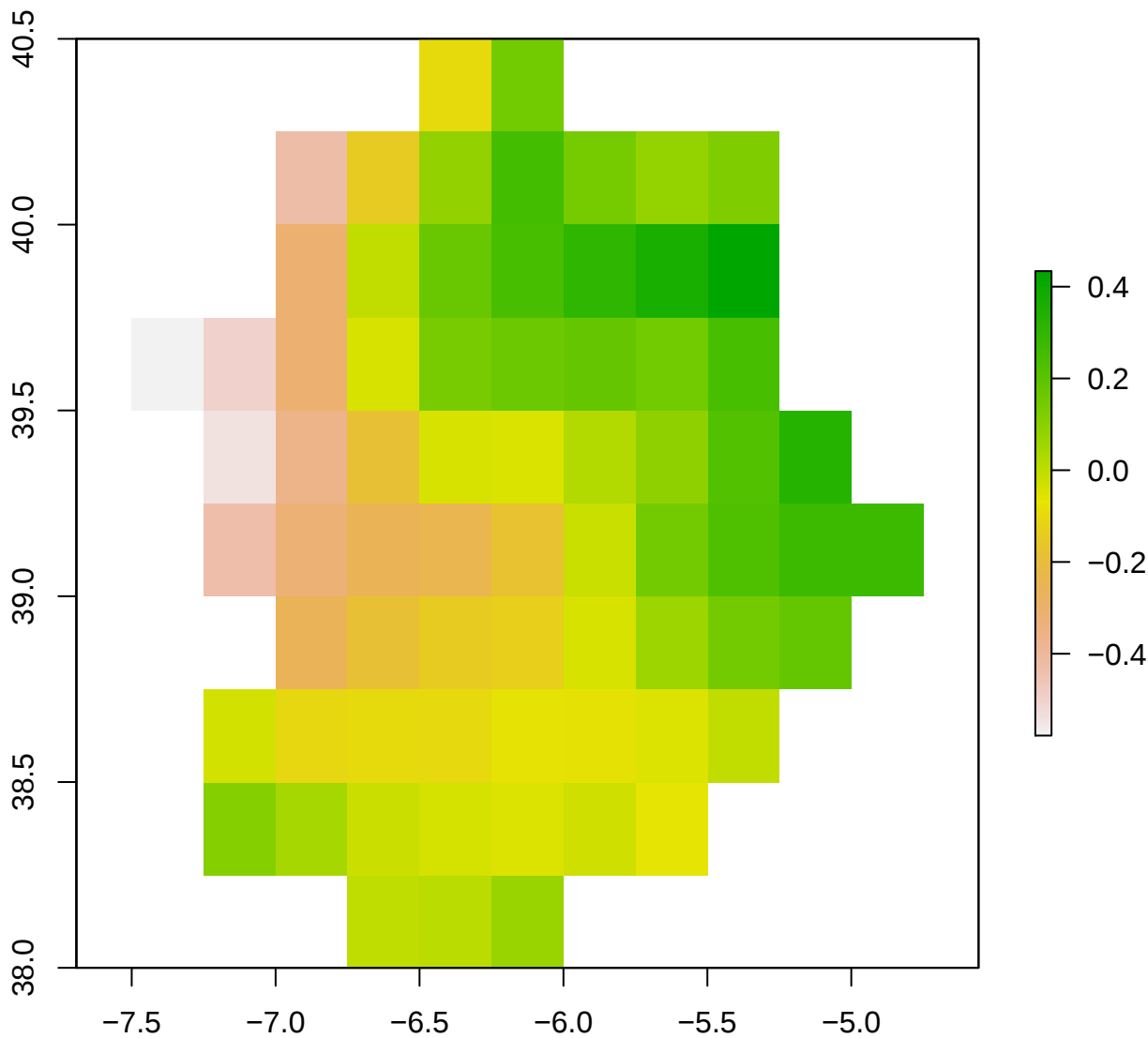
spi12_month - ES43 2008-04-01
