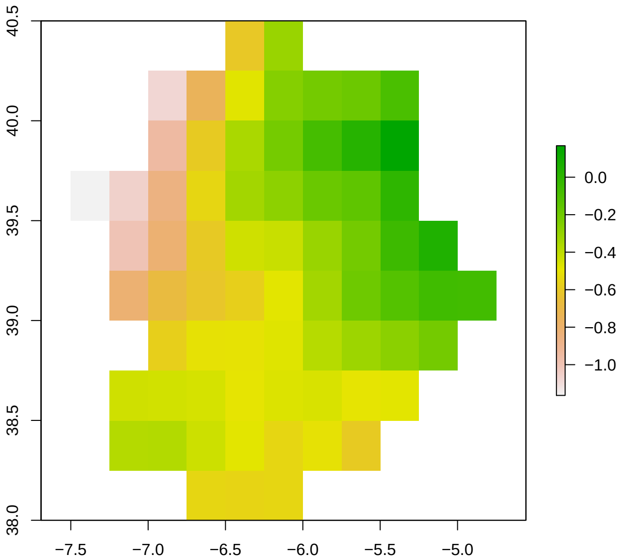
spi12_month - ES43 2008-03-01
