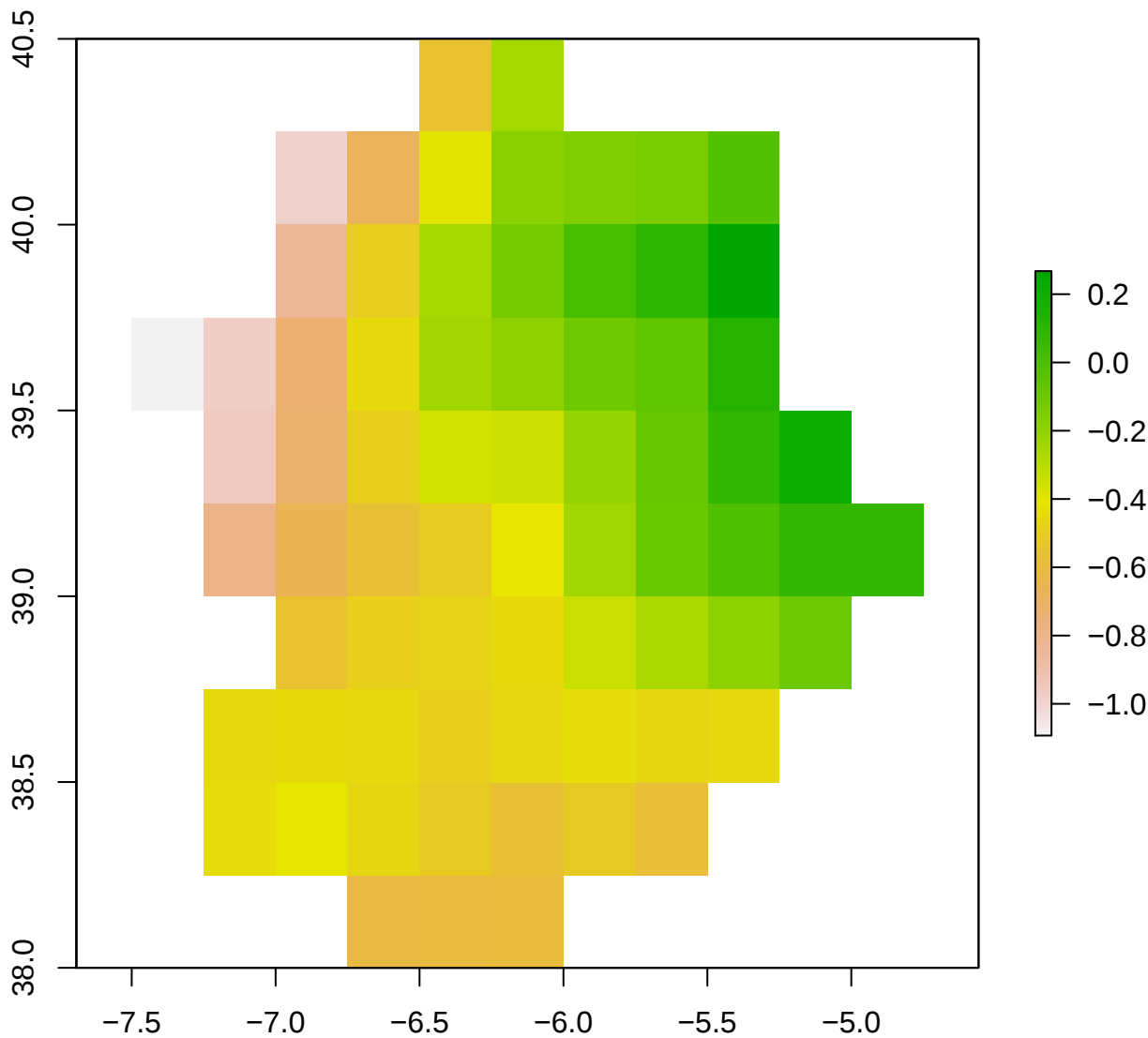
spi12_month - ES43 2008-02-01
