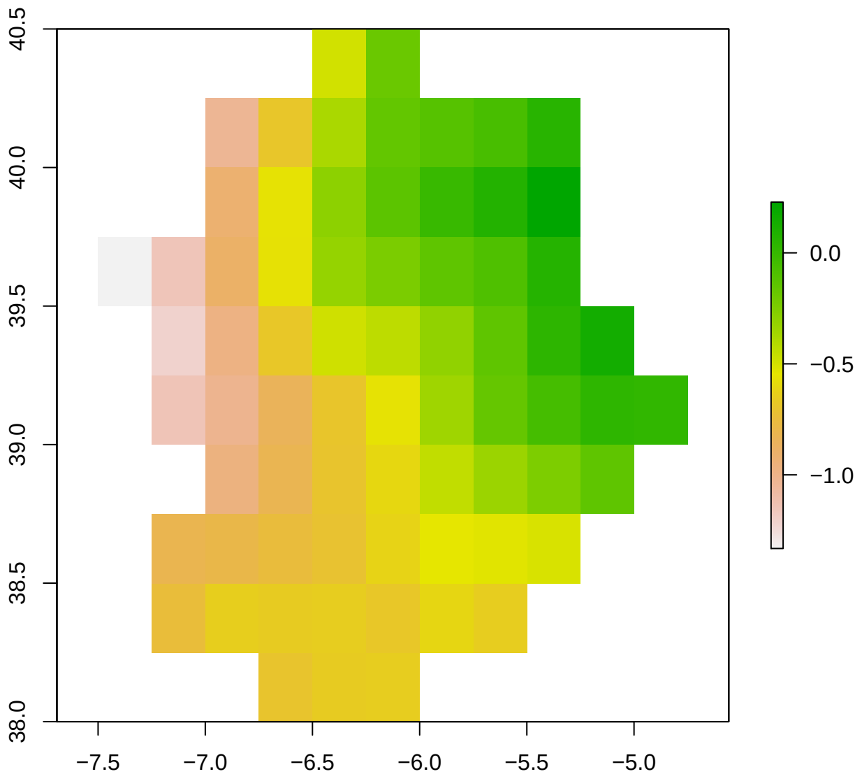
spi12_month - ES43 2007-12-01
