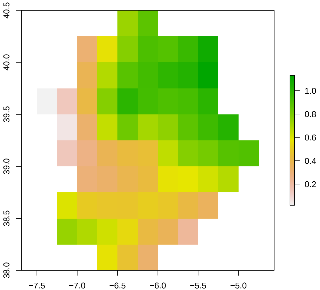
spi12_month - ES43 2007-09-01
