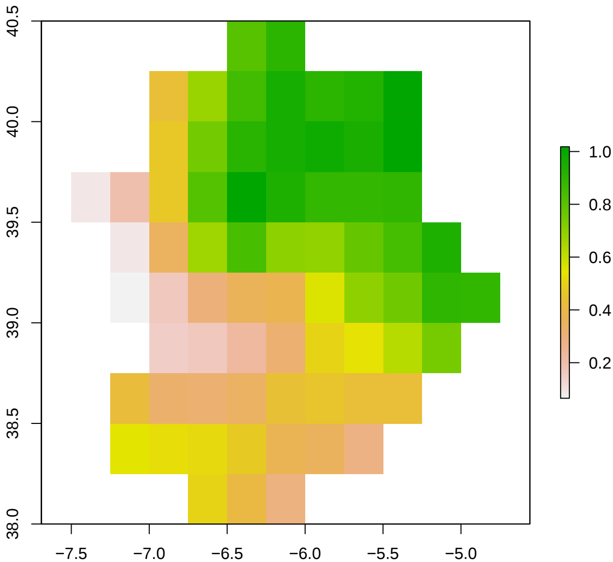
spi12_month - ES43 2007-06-01
