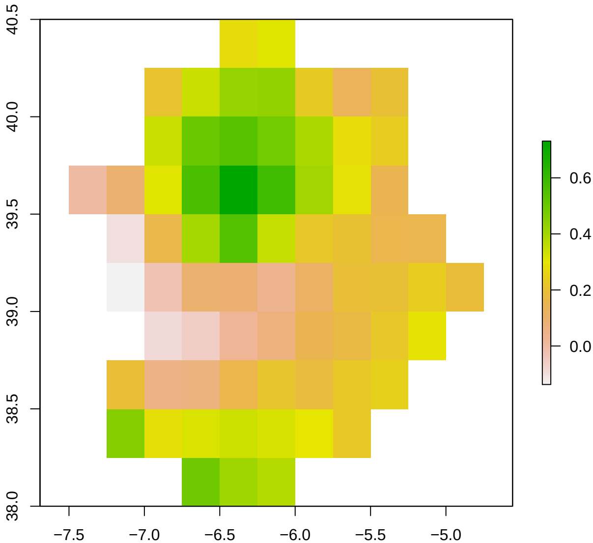
spi12_month - ES43 2006-12-01
