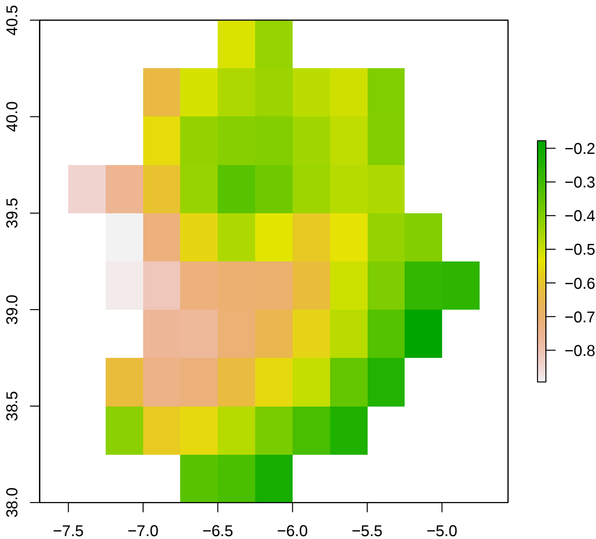
spi12_month - ES43 2006-10-01
