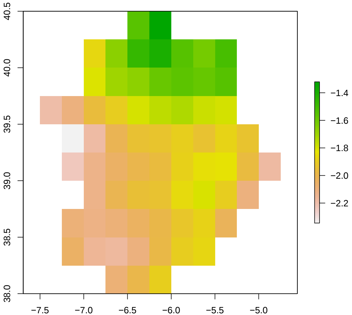
spi12_month - ES43 2005-12-01
