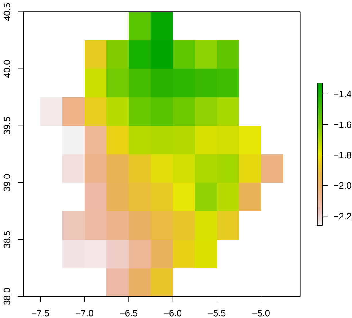
spi12_month - ES43 2005-10-01
