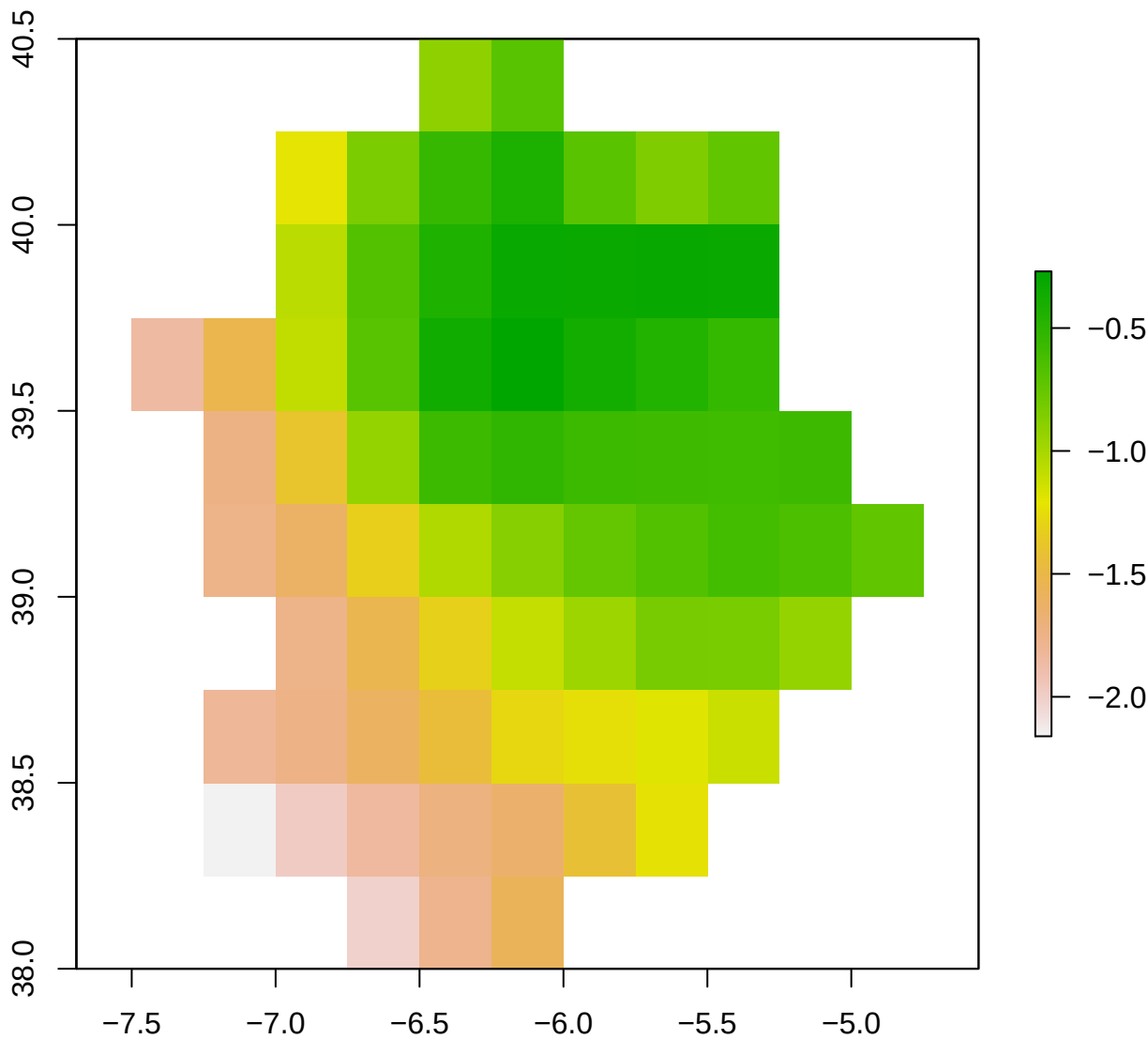
spi12_month - ES43 2005-03-01
