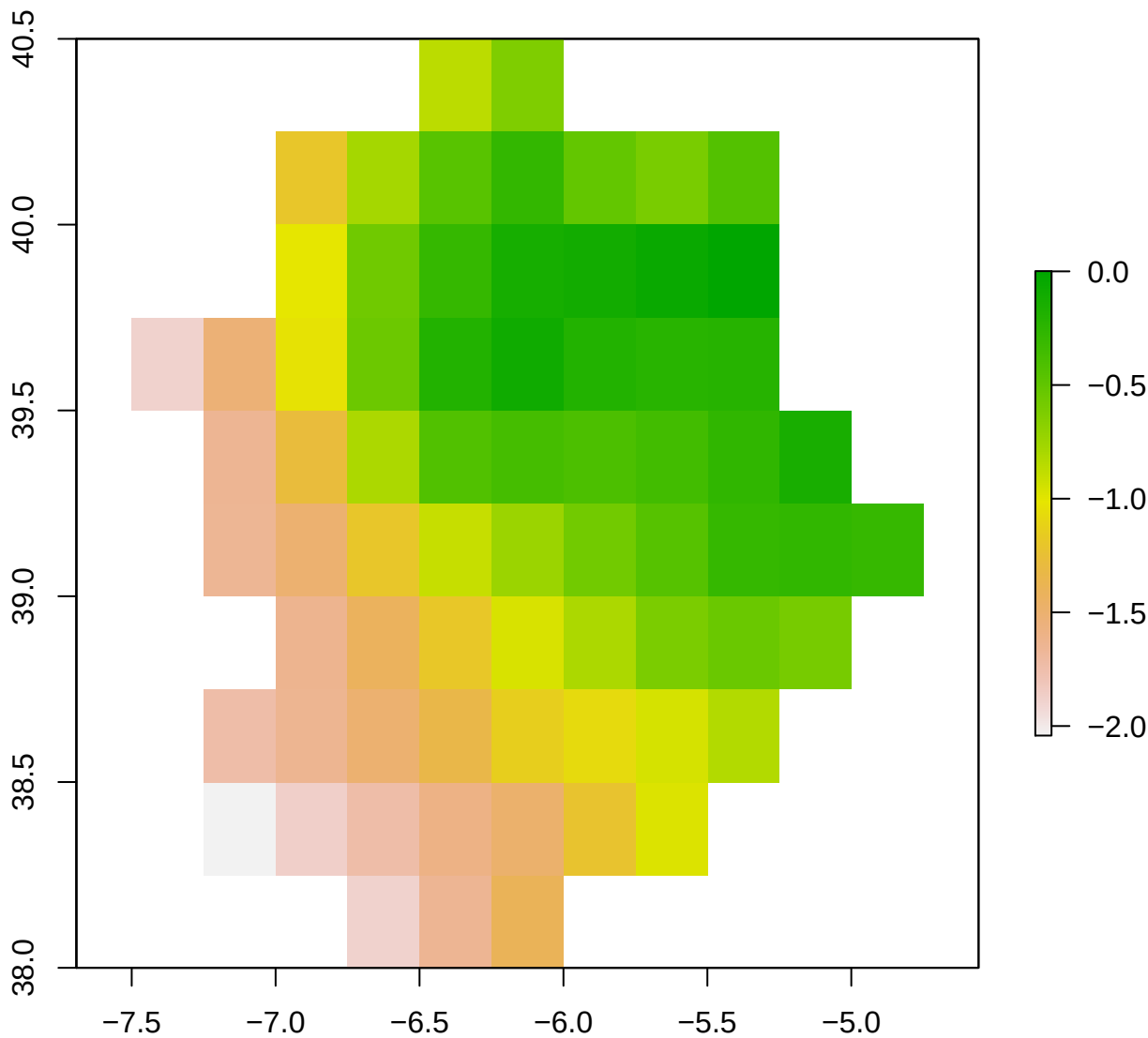
spi12_month - ES43 2005-02-01
