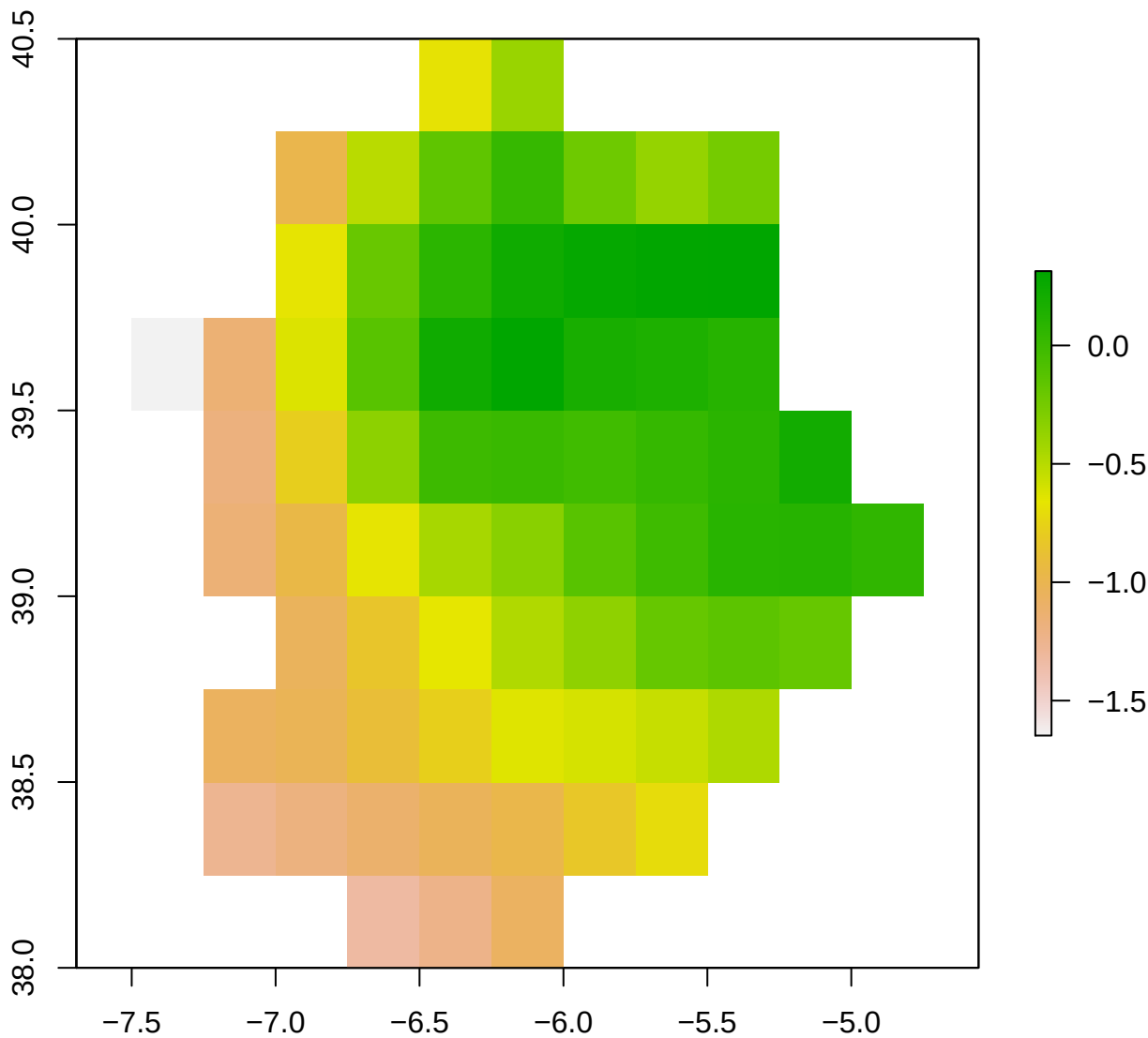
spi12_month - ES43 2005-01-01
